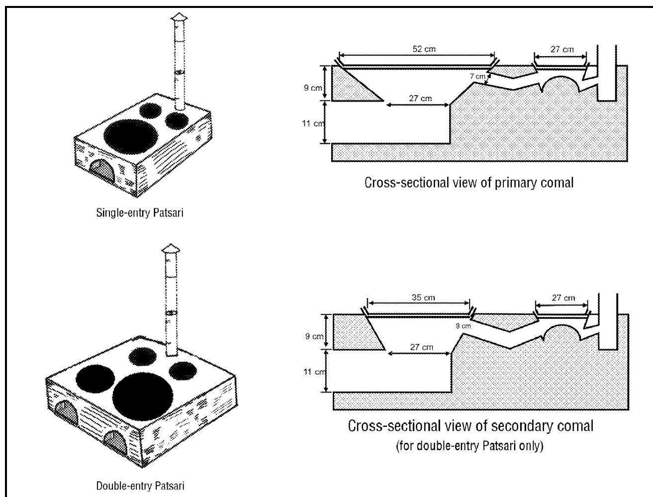
Figure 3. Top view and cross-sectional view of the two Patsari cookstove models
